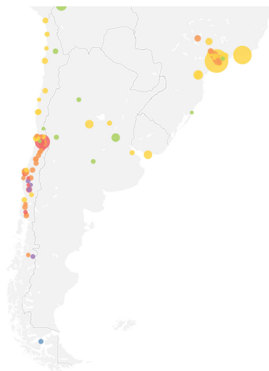
City markers indicating 2021 PM2.5 levels, size adjusted for population
