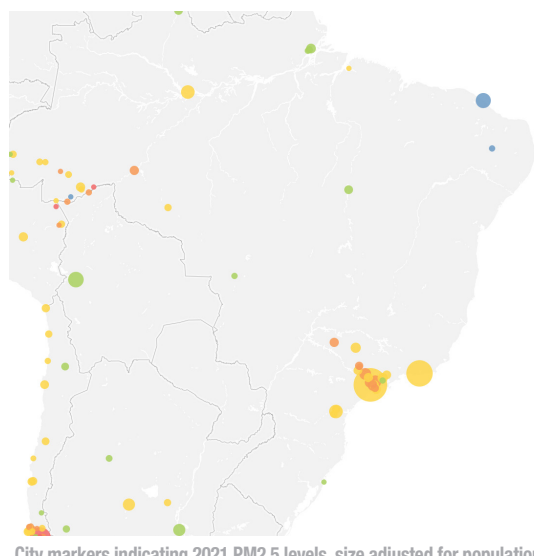
City markers indicating 2021 PM2.5 levels, size adjusted for population
