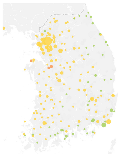
City markers indicating 2021 PM2.5 levels, size adjusted for population
