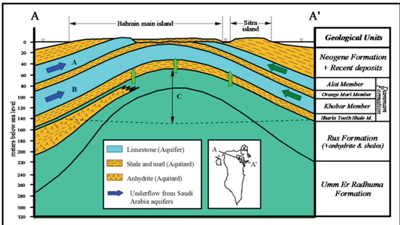
Fig. 4 Schematic Hydrogeological cross section for Bahrain Groundwater system (Zubari 1999). The colors of the zones denote the salinity categories: blue=relatively freshwater inflow from Eastern Saudi Arabia in the A and B aquifers; light green=brackish groundwater in
